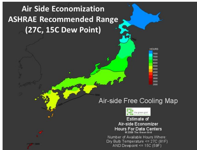
Figure 6. Air-side free cooling map of Japan (27°C with a 15°C dew point)
